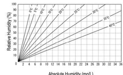
Fig. 2 Relative Humidity vs. Mass of Water Vapour
