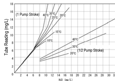
Fig. 1 Temperature Correction Chart 1 and 1/2 pump strokes
